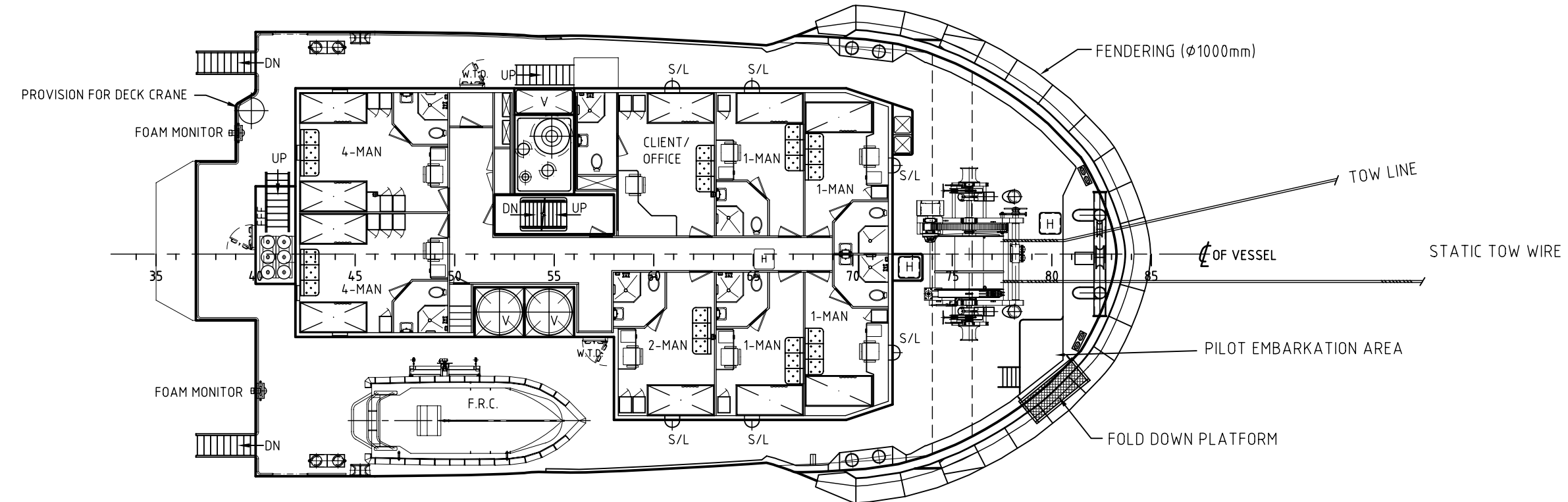
FORECASTLE DECK
