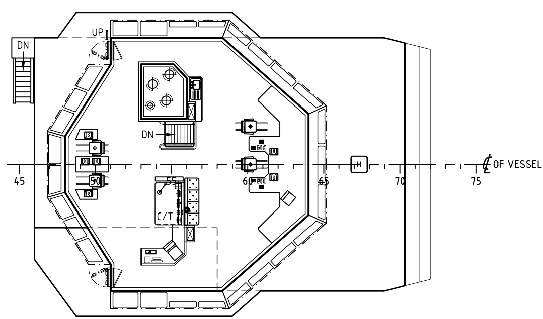
WHEELHOUSE DECK
