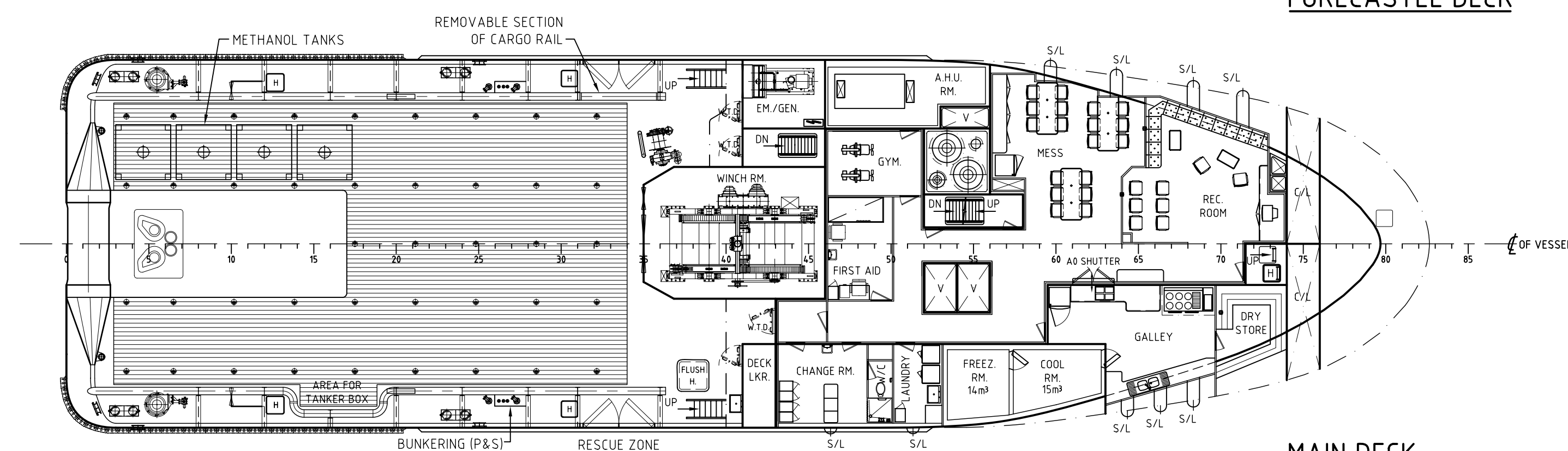
MAIN DECK
