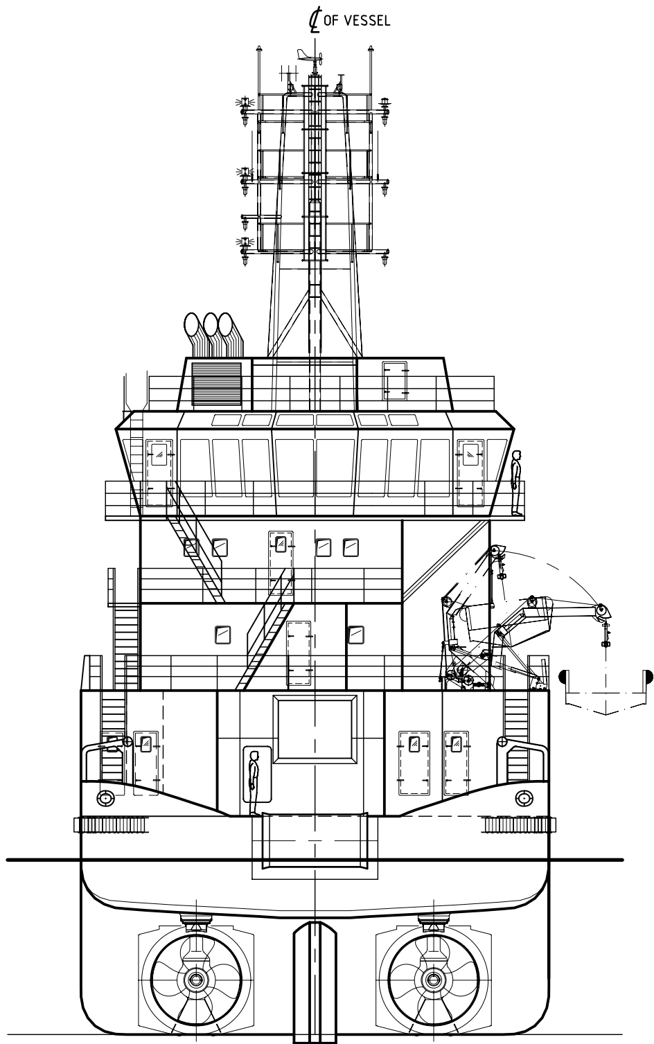
STERN VIEW
