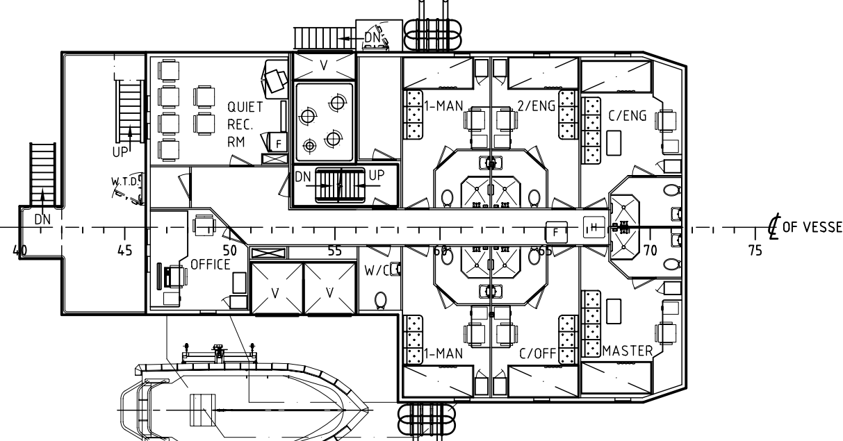
1 DECK
