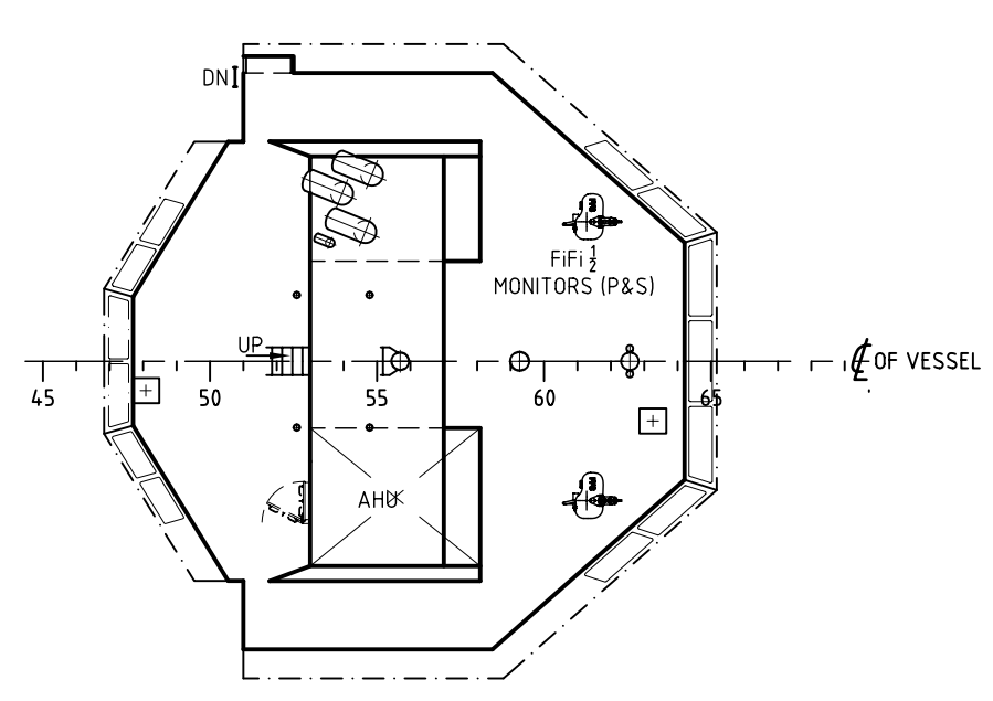
WHEELHOUSE TOP
