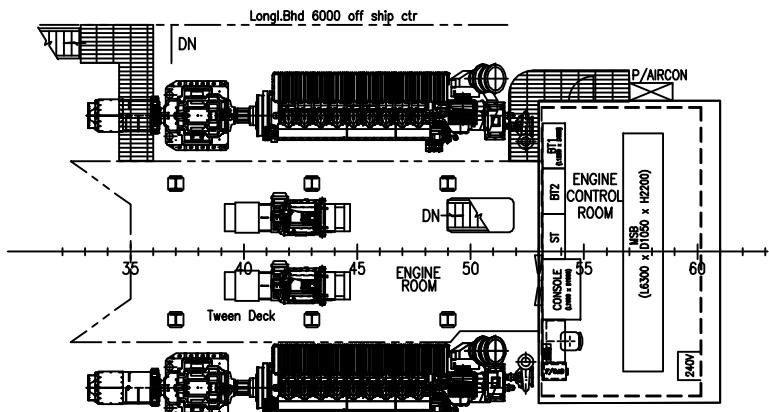
TWEEN DECK (ENGINE ROOM)
