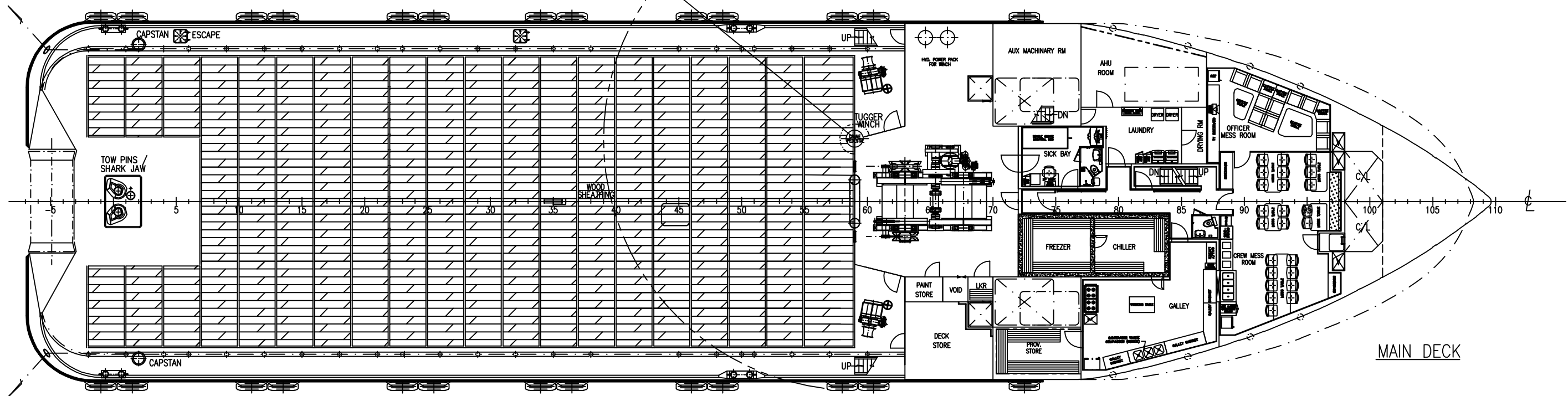
FORECASTLE DECK 16 x 2 MEN = 32 MEN TOTAL = 32 MEN
