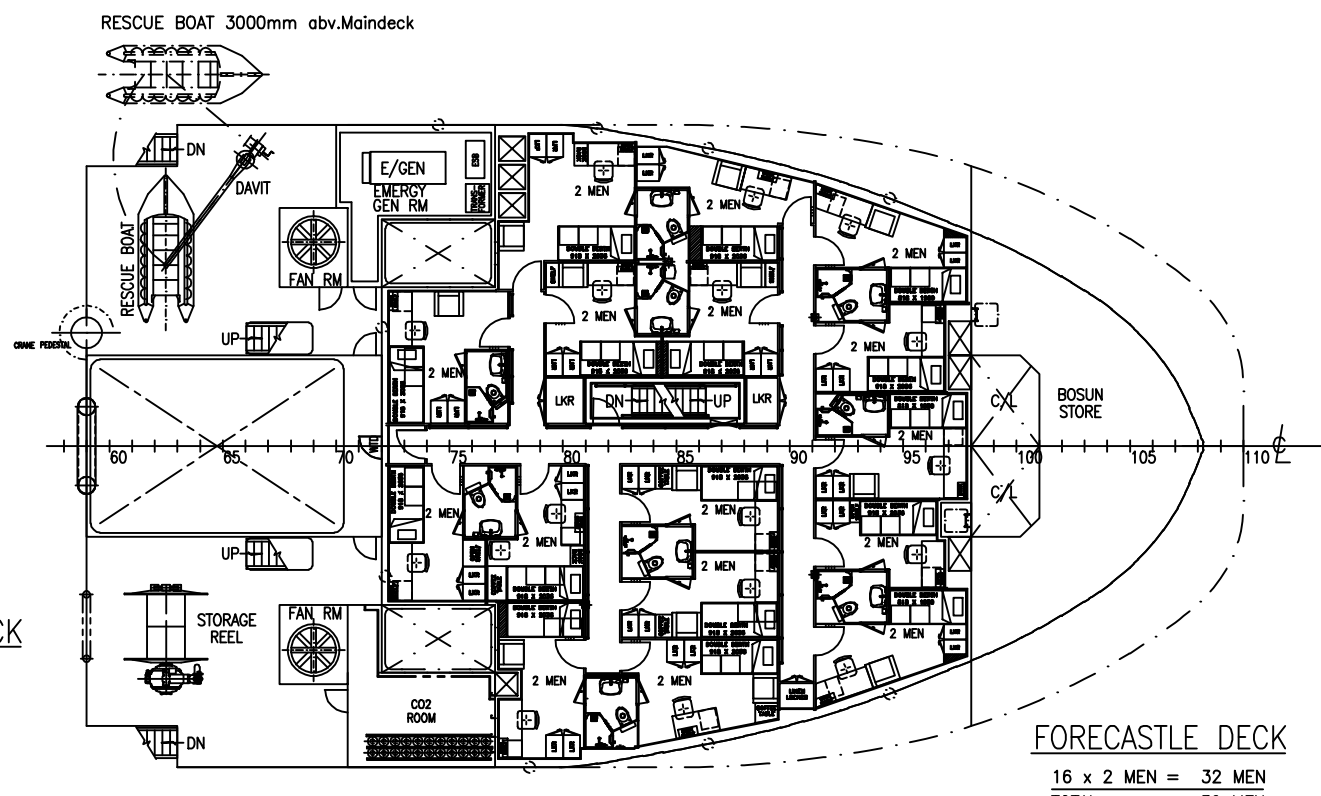
UPPER FORECASTLE DECK 3 x 1 MEN = 3 MEN 4 x 2 MEN = 8 MEN TOTAL = 11 MEN
